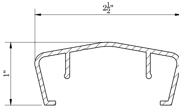
TOP CAP STYLE 1
