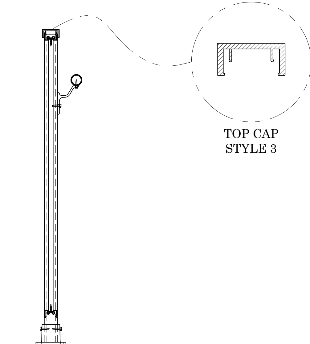
CUT-SECTION
